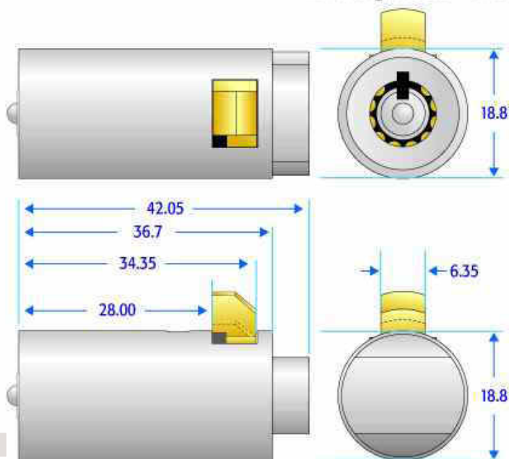
Locking Insert - T8871
